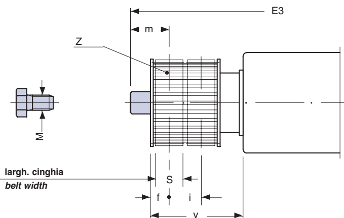
PULEGGIA DENTATA TOOTHED PULLEY
